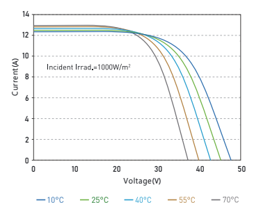
I-V Curve at Different Temperature (470W)
