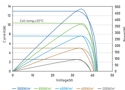
I-V/P-V Curve at Different Irradiation (470W)
